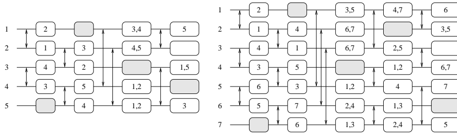
Figure 2: Gossiping among 5 vertices in 4 rounds and 6 steps (left) among 7 vertices in 5 rounds and 8 steps
