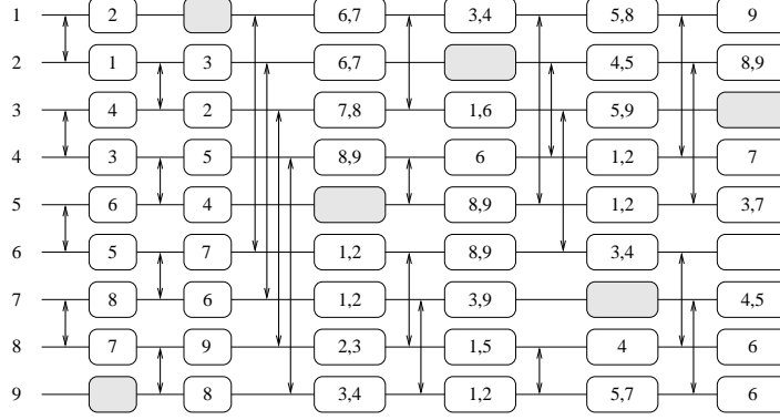
Figure 3: Gossiping among 9 vertices in 6 rounds and 10 steps
